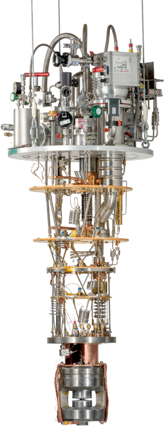
Internal view of the dilution cryostat developed by the ILL team. The VX5 Paris-Edinburgh press is suspended from or attached to the stage of the mixing chamber with a support made from OFHC copper.
