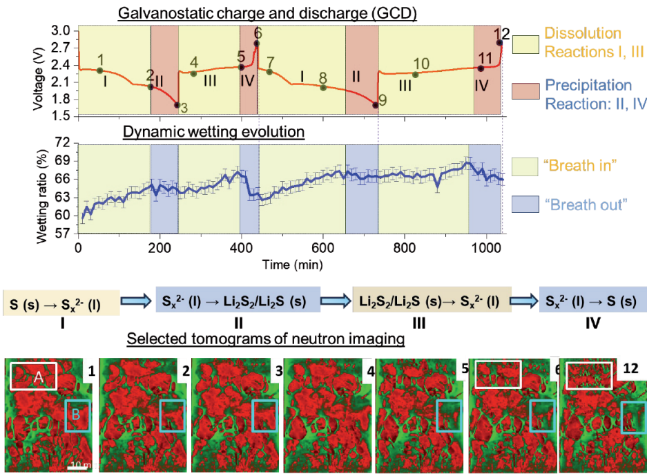
Figure 1: The dynamic electrolyte wetting is correlated to the discharge/ charge processes of the Li-S pouch cell. The selected tomograms demonstrate the wetting evolution in local areas (e.g. the area marked A and B).
