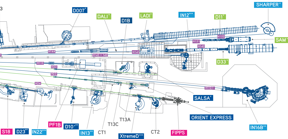
NEUTRON GUIDE HALL ILL7 - VERCORS SIDE (WEST)
