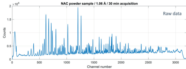
Diffraction line-profile from a NaCaAlF powder sample acquired with the new Trench-MWPC detector on the D20 instrument.
