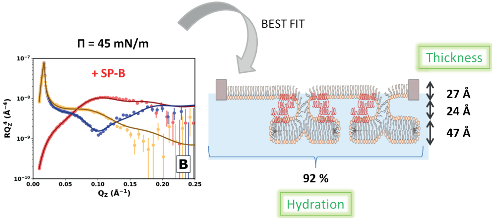
Figure 1: Neutron reflectivity profiles obtained for hydrogenous lipids + SP-B in D 2 O (yellow), deuterated lipids + SP-B in D 2 O (blue) and deuterated lipids in ACMW (red) at 45 mN/m. The lines show the fits to a model that describes the structure of the interfacial film as a 27 Å monolayer, a 24 Å hydrated gap attributed to the presence of SP-B, and a 47 Å bilayer connected to the interface thanks to the protein.
