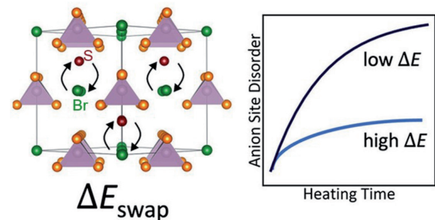
Figure 1: Schematic illustration of anion site swapping in lithium argyrodites and its kinetic consequences. The left panel shows sulfur and bromine exchanging between crystallographic sites, characterised by an anion swap energy barrier, \Delta E_{\text{swap}} . The right panel illustrates how this barrier controls the rate at which anion disorder develops during heating: low \Delta E leads to rapid disordering, while high \Delta E results in slower, incomplete disorder frozen into the final structure.
