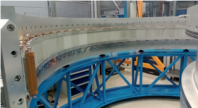
Inside view of the D20 trench-MWPC detector. The 25 trench modules are mounted side by side without any dead zone to ensure a continuous 160° angular coverage.
