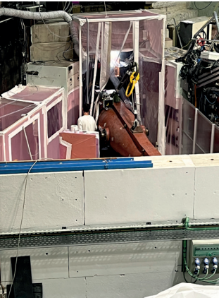
Work on beam tube H13.
