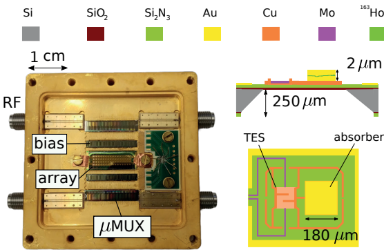
Figure 2: Left: Copper box containing the 64 TES array in the middle. The two chips on either side of the array are the bias network and the microwave multiplexer (μMUX, developed by the National Institute of Standards and Technology, Boulder, USA), respectively. Right: Schematic, not to scale, representation of the HOLMES TES microcalorimeter used in the experiment.
