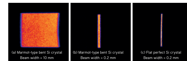
Figure 2: Hard X-ray diffraction images of a Marmot-type Si crystal ( R = 2.6 m). (a) Uniform curvature observed using a large beam width (10 mm). (b) Preserved structural quality with a small beam width 0.2 mm. (c) Diffraction image of a perfect flat Si crystal with a small beam (0.2 mm) for comparison.
