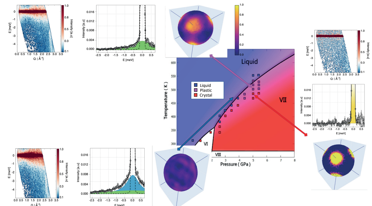
Figure: Pressure–temperature phase diagram of water in the investigated region, highlighting the stability fields of the liquid (blue), plastic crystal (purple), and ordinary ice VII (red). Symbols indicate the thermodynamic points explored by quasi-elastic neutron scattering. Representative measurements of the dynamical structure factor S(Q, \omega) and their energy projections are shown for the three phases. In the liquid phase (bottom), both translational and rotational contributions are observed. In the plastic phase (top), translational diffusion is arrested while fast rotational dynamics persist on the picosecond timescale. In ordinary ice VII (right), no quasi-elastic broadening is detected within the instrumental resolution. The three-dimensional maps illustrate the orientational probability distribution of hydrogen atoms as calculated by Molecular Dynamics simulations, highlighting the dynamically disordered nature of the plastic phase despite the preservation of an average orientation along the cubic lattice diagonals.
