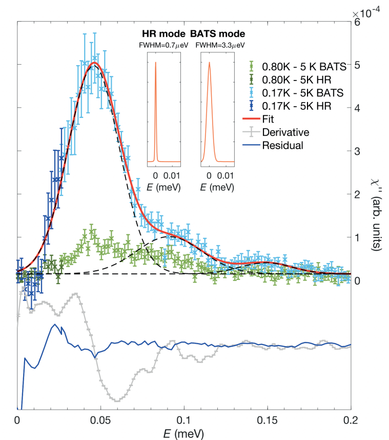
Figure 2: Imaginary part of the dynamical spin susceptibility from experiments on IN16B. The continuous red line is a fit using a constant background and three Gaussian peaks. The insets show the energy resolution provided by each instrument configuration.
