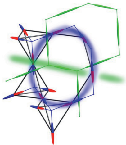
Figure 1: Magnetic moments (blue/red ellipses) on a pyrochlore lattice (in black) constrained by a local ‘2-in-2-out’ rule, defining flux sources that form a diamond lattice (in blue). Quantum dynamics on rings create emergent flux variables (in green) living on a second diamond lattice.
