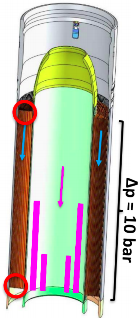
Figure 3.1: Fuel element vertical section. The control rod (pink) is extracted downwards and causes two hotspots (red) at the fuel extremities
