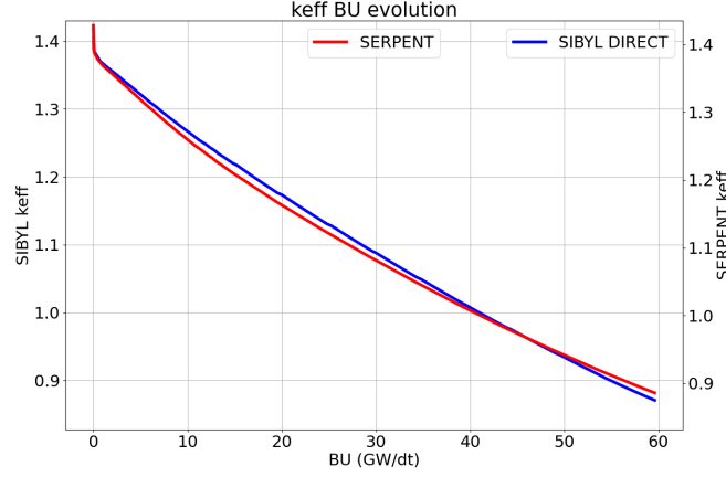
Figure 3.18: SIBYL results comparison with SERPENT: UAM multiplication factor evolution
