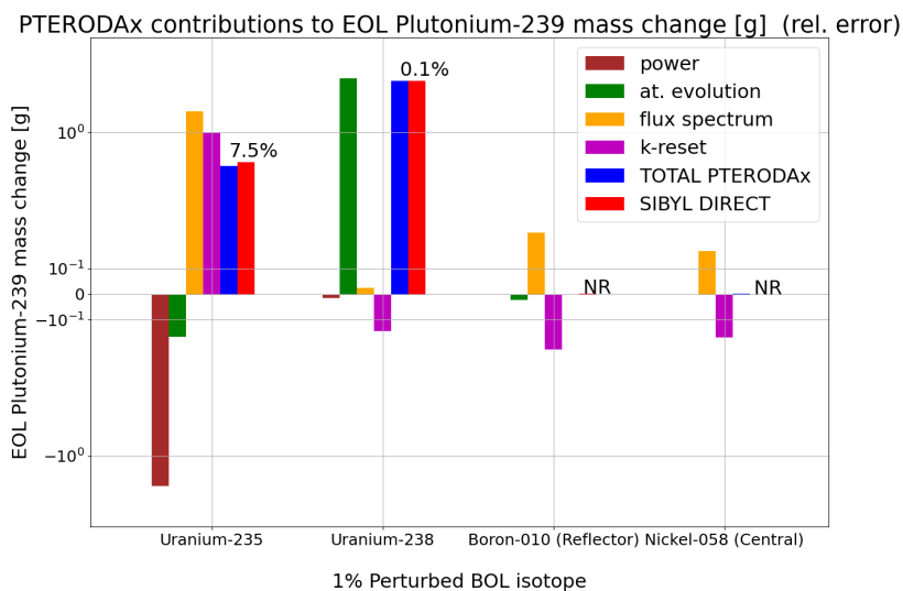
Figure 4.16: PTERODAx results for EOL Pu-239 sensitivity to different BOL perturbations, compared with SIBYL direct calculations performed with criticality reset
