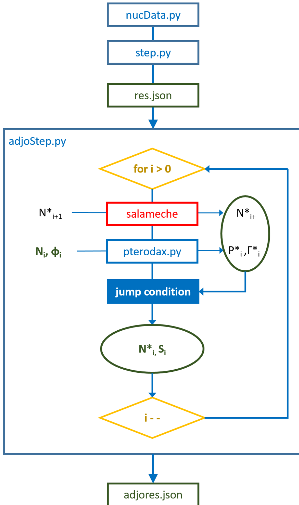
Figure 3.19: Python architecture
