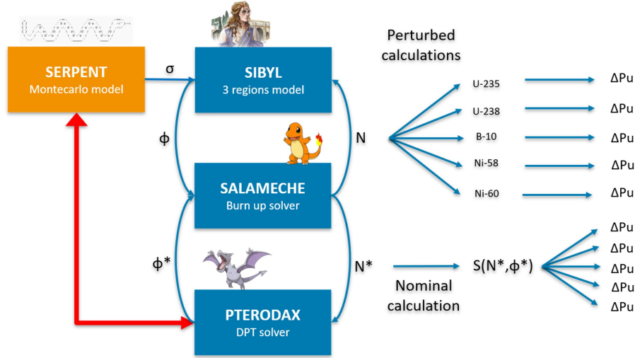
Figure 4: Python architecture
