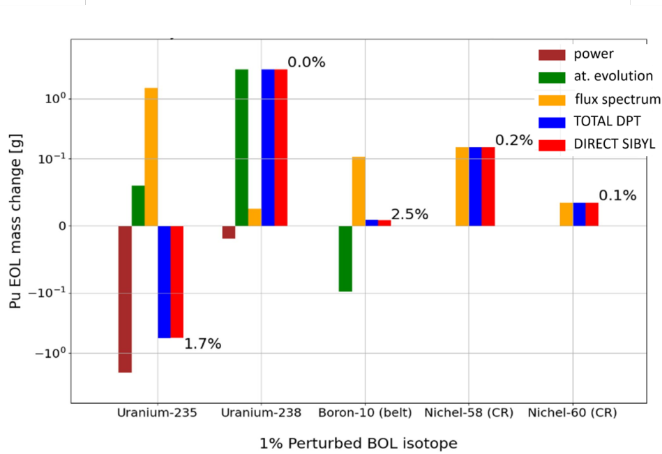
Figure 4.13: PTERODAx results for EOL Pu-239 mass sensitivity to different BOL perturbations, compared with SIBYL direct calculations (the relative error is reported on top of the histograms)
