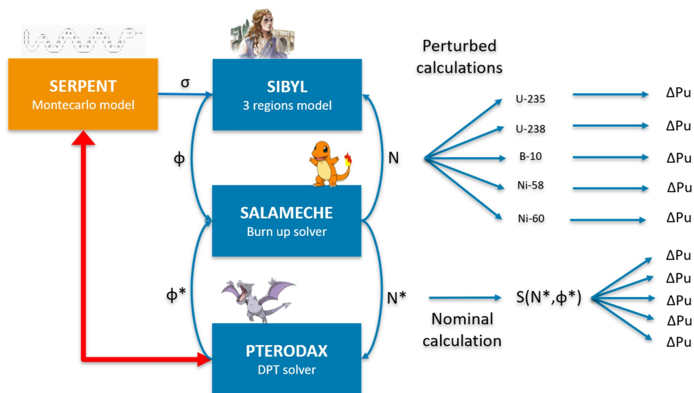
Figure 3.20: Python architecture
