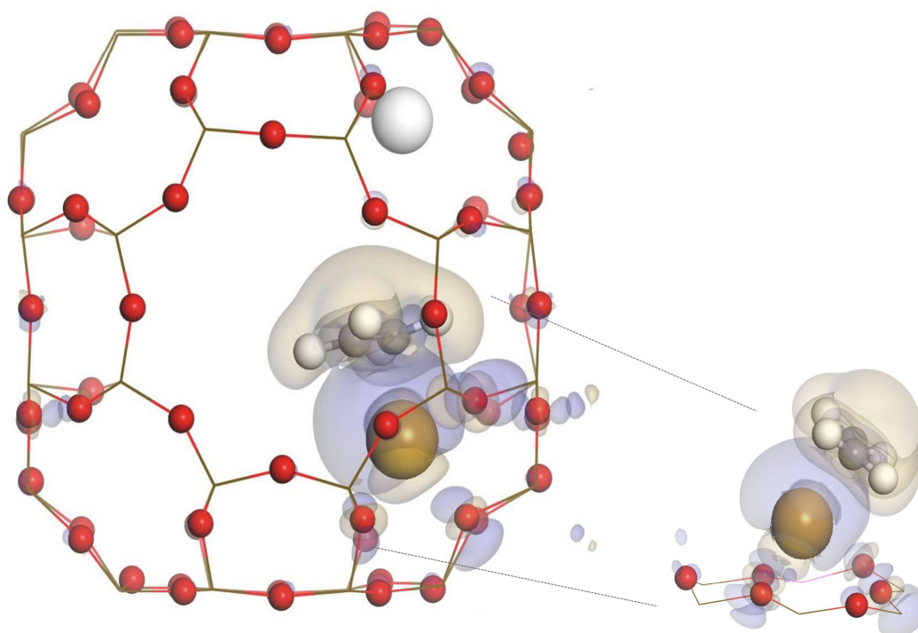
Figure 3.23: Isosurfaces created for -8.369\text{e}\text{\AA}^{-3} , representing the electron density difference between ethylene and HAg-LTA. The yellow shade represents areas of charge depletion while the blue one, of charge accumulation. This rearrangement is attributed to \pi -complexation interaction. The picture illustrates the full contribution of the HAg-LTA lattice atoms and the molecule.
