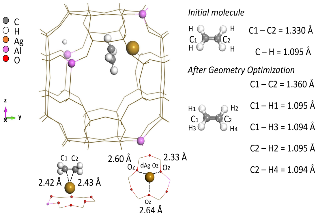
Figure 3.21: Structural details of lta cage in the energy minimized C 2 H 4 HAg- LTA model. The distances between Ag and the closest framework oxygen atoms, d_{\text{Ag-Oz}} , as well as Ag-C, d_{\text{C-Ag}} are shown. C 2 H 4 molecule is represented before and after the system energy minimization with its corresponding C-H distances, d_{\text{C-H}} . Al, Ag, C and H atoms are indicated in the figure. O atoms are highlighted in the 6-ring where Ag cation is placed, O z are the 6-ring Oxygen atoms closest to Ag. Si and O atoms of lta cage are represented by brownish lines to facilitate Ag-C 2 H 4 complex visualization. The complex lies in a region called 8-ring pocket.
