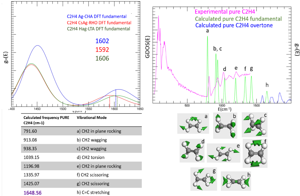
Figure A.7: C=C stretching calculation by comparing calculated C=C stretching frequency of C 2 H 4 with the calculated C 2 H 4 adsorbed on each Ag-zeolite. These values are \approx 46 \text{ cm}^{-1} for Ag-CHA, 56 \text{ cm}^{-1} for CsAg-RHO and 42 to Hag-LTA.
