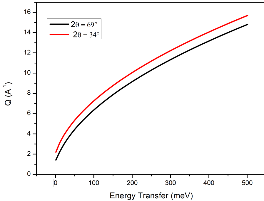
Figure 2.10: Kinematic range reached by the indirect geometry spectrometer (IN1-Lagrange) at final energy E_f = 4.5\text{ meV} . Scattering angles from 34 - 69^\circ , that corresponds to the two extreme values of the scattering angles on IN1-Lagrange.
