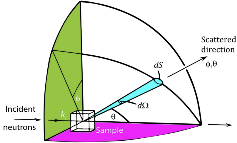
Figure 2.3: Representation of the scattering process. The incident neutrons interacts with a sample and some neutrons are scattered in the direction \phi, \theta , reaching a detector of small area ( dS ).
