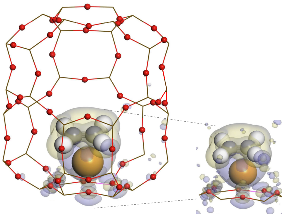
Figure 3.9: Isosurfaces created for -8.369\text{e}\text{\AA}^{-3} , representing the electron density difference between ethylene and Ag-CHA. The yellow shade represents areas of charge depletion while the blue one, of charge accumulation. This rearrangement is attributed to \pi -complexation interaction. The picture illustrates the full contribution of the Ag-CHA lattice atoms and the molecule.
