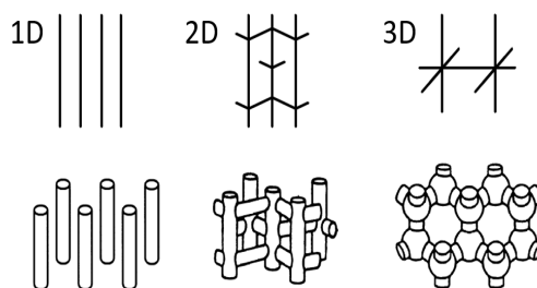
Figure 1.7: Classification of zeolites according to pore connectivity.
