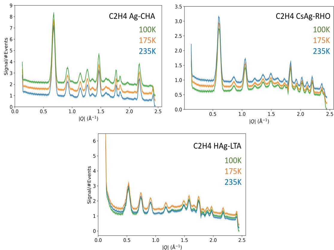
Figure A.31: Cuts of S(Q, \omega) along |Q| from 0 to 2.5 \text{\AA}^{-1} over energy values from -0.2 to 0.2 meV, representing S(Q) .
