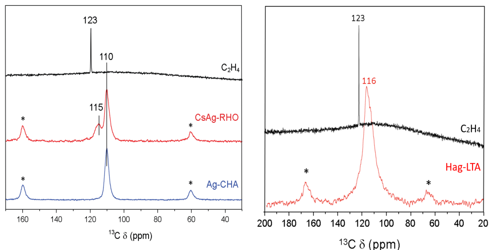
Figure A.3: ^{13}\text{C} MAS NMR spectra of free-ethylene gas compared to ethylene adsorbed on Ag-CHA, CsAg-RHO and HAg-LTA zeolites. Spinning rotation bands are indicated by asteriks (*).
