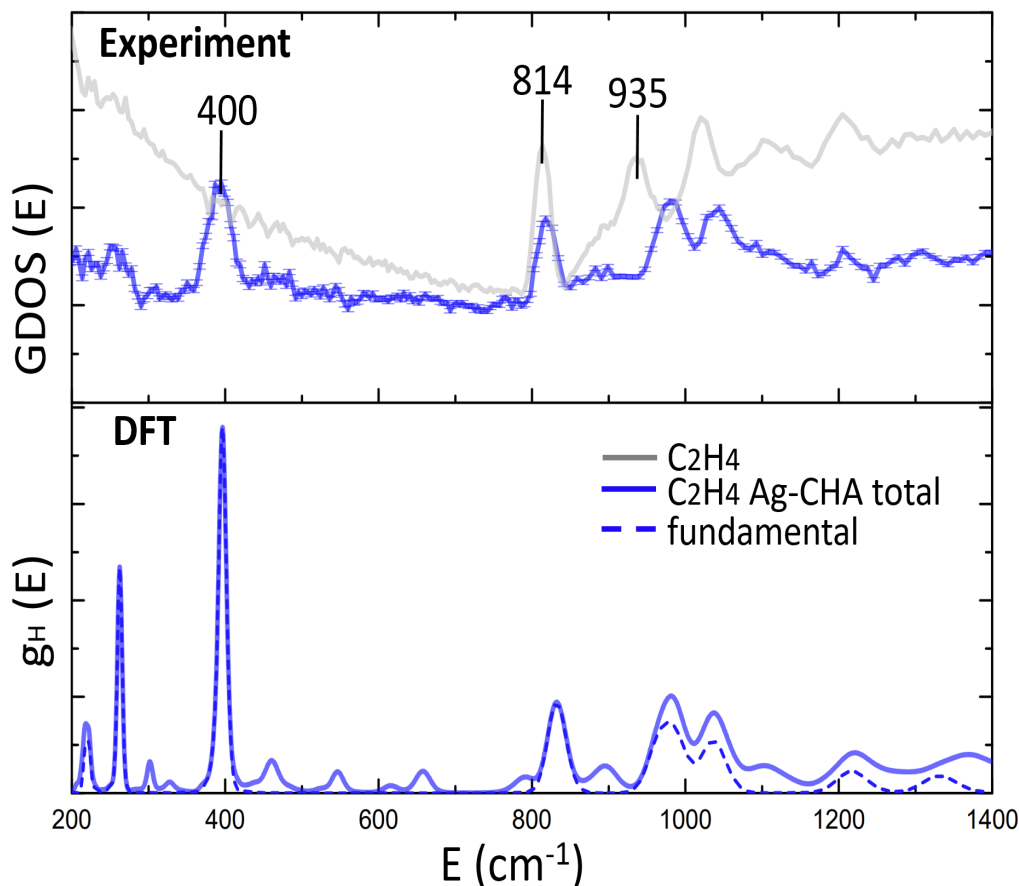
Figure 3.7: Comparison between experimental and calculated INS spectra, fundamental and total frequencies (considering first overtones), of C_2H_4 adsorbed on Ag-CHA with that of pure gas for reference.
