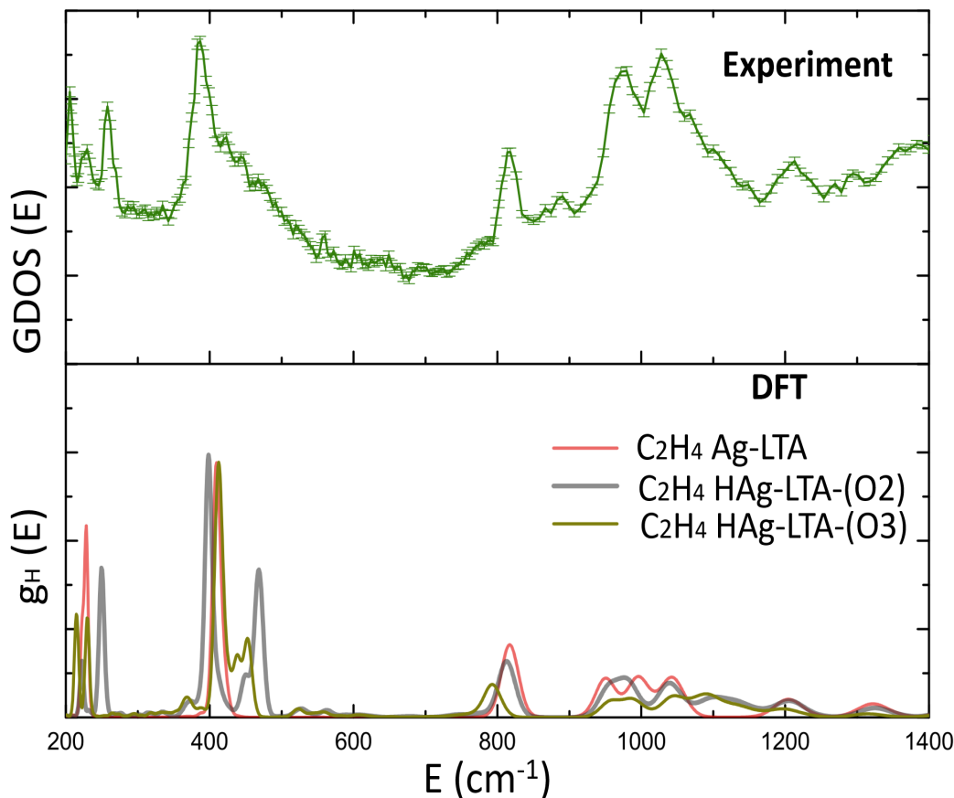
Figure 3.20: Comparison of the experimental INS spectrum of HAg-LTA sample with the calculated neutron spectra for all configurations considered: \text{C}_2\text{H}_4 Ag-LTA, \text{C}_2\text{H}_4 HAg-LTA-(O2) and \text{C}_2\text{H}_4 HAg-LTA-(O3), with fundamental frequencies.
