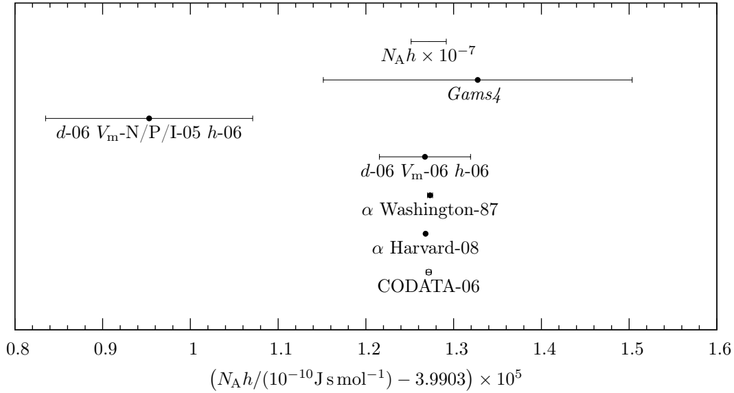
Figure 1.11: Values for N_A h . All “-06” values are the recommended values by CODATA-06, where d indicates the \{220\} lattice parameter, V_m the molar volume of natural silicon and h the Planck constant. Values derived from \alpha are converted using (1.6) and the CODATA values for R_\infty and A_r(e) . The value Gams4 is extracted from [Rai+05], assuming the correctness of E = mc^2 . V_m -N/P/I-05 is the value coming from the XRCd method [Fuj+05]. Its weight for the CODATA adjustment was obviously negligible.
