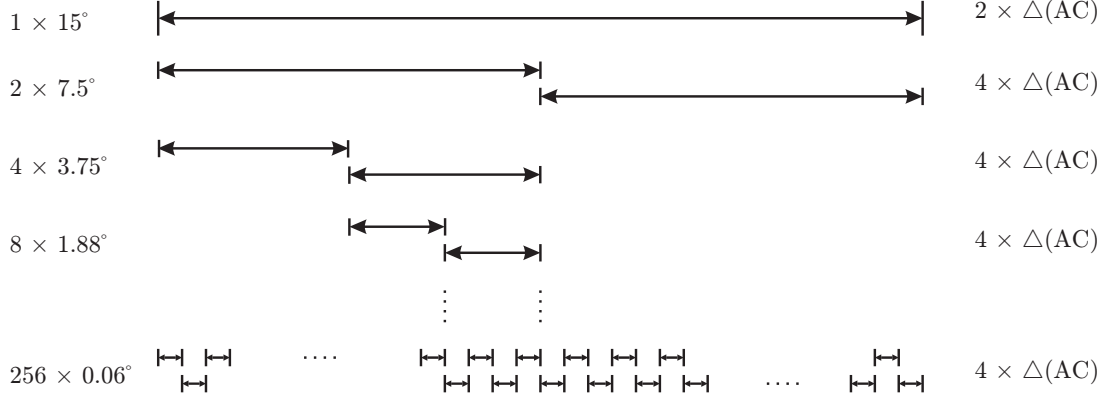
Figure 2.19: Non-linearity mapping: An angle of 15^\circ is continuously subdivided into 15^\circ/2^8 . Any subdivision introduces the autocollimator uncertainty U(\text{AC}) as many times as it has to be measured. Hence every range of 0.06^\circ can be linked to the full 15^\circ range with 2 + 4 \times 8 autocollimator measurements.
