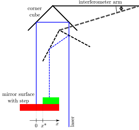
Figure 2.15: Surface-step illustration. One corner cube is sketched in symmetric position and at a large angle. The laser beam gets displaced. Hence during an axis rotation the laser scans the surface of the mirror. If the latter is not perfectly flat the interferometer readout will depend on the surface, and not only on the rotation.
