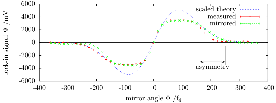
Figure A.7: Autocollimator asymmetry and comparison with theory. A copy of the data is mirrored at the origin to illustrate the asymmetry in the region around +200 f_4 . The theory was scaled to the data by fitting to the data range -380 to +40 f_4 . The discrepancy at high signal may be due to saturation of the photo detector or the lock-in amplifier and was not further investigated. The signal was measured without amplification, and is thus about 10 times smaller than usual. For better comparison, it was scaled back. The reason to do so is the saturation limit of 10 V of lock-in amplifier and analogue-to-digital converter.
