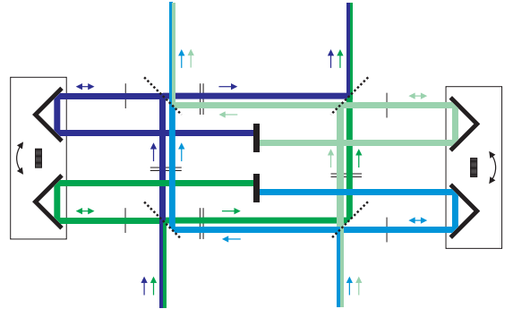
(b) Layout for two sides or axes. The same polarizing mirrors are used for both sides. A second laser also providing two frequencies—again separated by polarization—is injected at a different spot. It may be a copy of the first one, created by a non-polarizing beam splitter. Beams for left and right axis may overlay.
