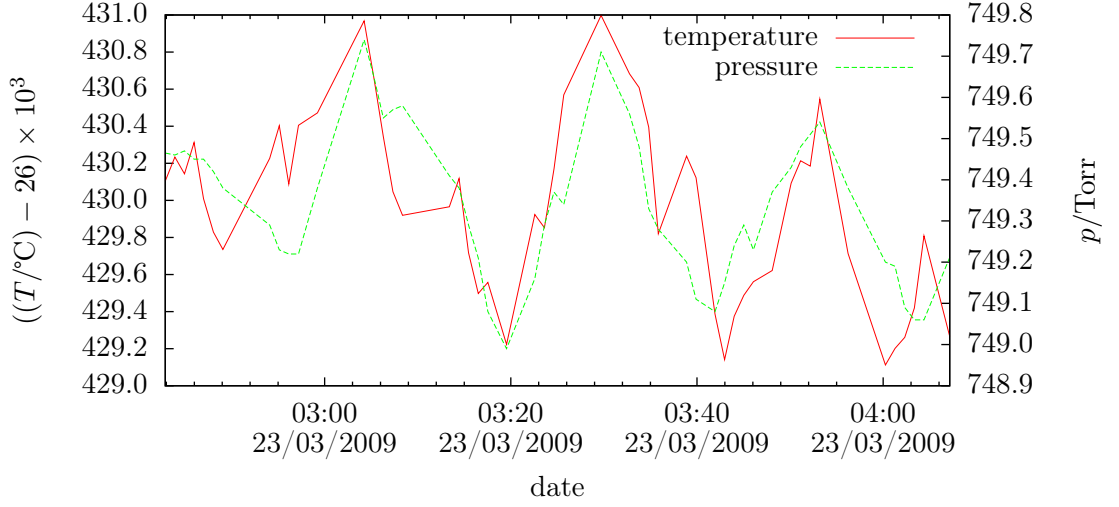
Figure 3.18: Adiabatic pressure oscillation inside the reactor building cause temperature oscillation. The temperature T oscillates with an amplitude of 1 mK, the pressure p with 0.7 Torr which is 1 mbar. The oscillation period is about 1500 s.
