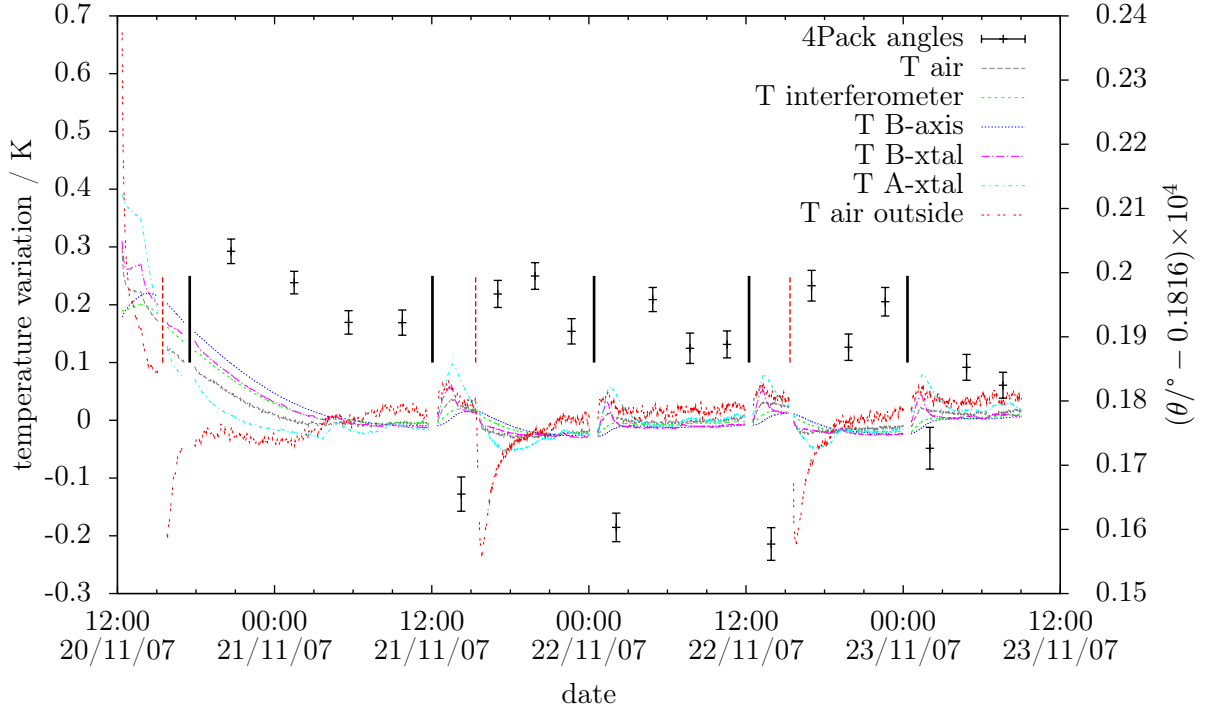
Figure 3.14: Influence of thermal variations on instrument instability. The temperature is perturbed by the filling of the Germanium-detector (vertical line, red dashed), and – more important for the instrument stability – by reference scans (vertical line, solid black). Therefore, this whole data set has been disregarded.
