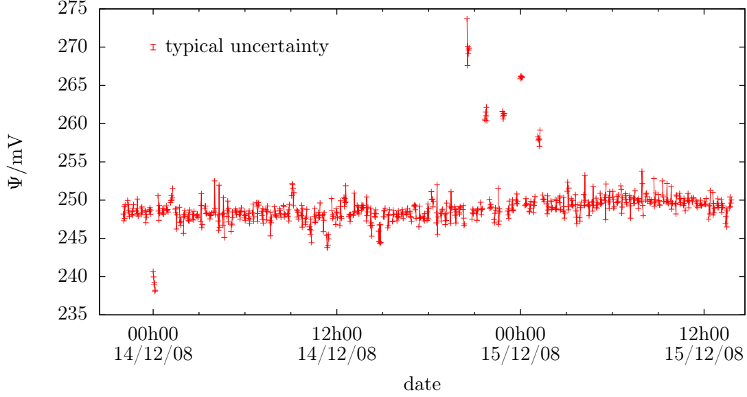
Figure 3.2: The autocollimator offset monitored during a full calibration. If any mirror was in the range of the autocollimator, the sample was excluded and the line in the graph interrupted. The voltage was sampled with 10 Hz. Each data point is the average over 500 samples.
