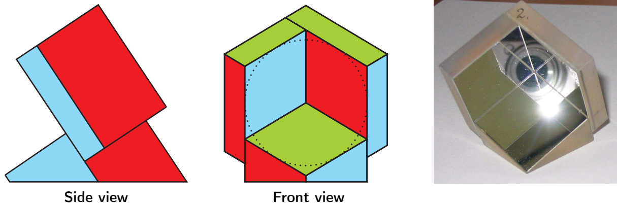
Figure 4.12: Scheme and photograph of the corner cube. Parallel surfaces are drawn in same colour. The aperture is 42 mm.
