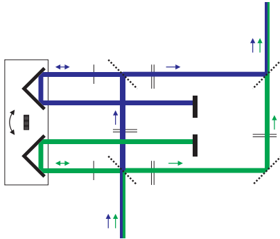
(a) Interferometer layout for one side or axis only. It is a combination of Michelson and Mach-Zehnder interferometer. The laser is injected at one spot; the two frequencies must be separated by perpendicular polarization.
