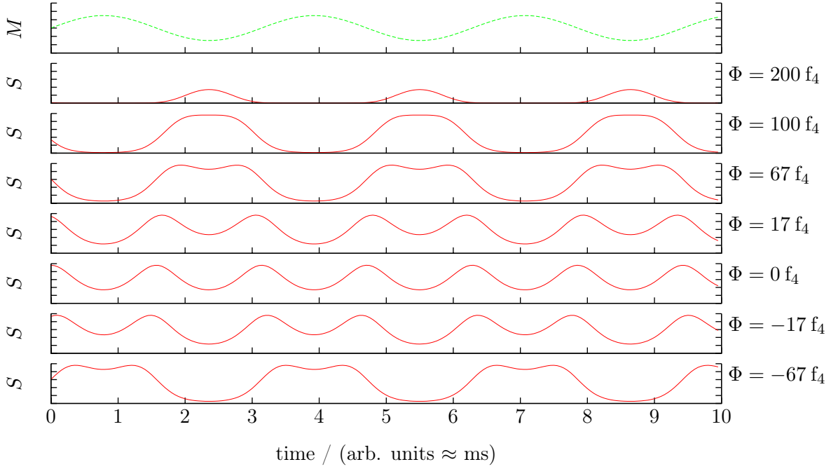
Figure A.6: Autocollimator signal –calculated from theory. The topmost graph shows the induced wobbler mirror oscillation, below are the detector signal on different angles of the polygon mirror. Note the increase of the signal in the far approach ( \Phi \approx 200 f_4 ). Important for the position sensitivity is the phase change at \Phi = 0 f_4 . All axes are in arbitrary scale.
