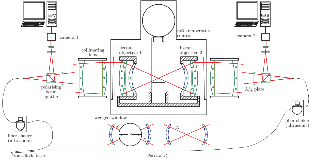
Figure 1.8: Principle of the Fizeau interferometer to determine the diameter of the SI sphere. Drawing from [Nic09].
