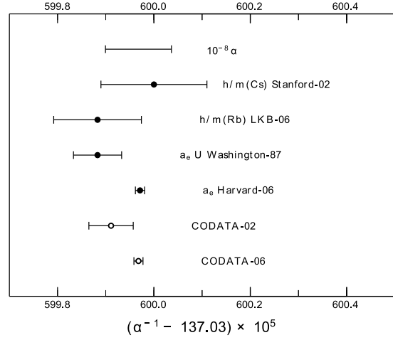
Figure 1.2: Values of the fine-structure constant \alpha with u_r < 10^{-8} , in order of decreasing uncertainty from top to bottom. The data are identical to those in Figure 1.1.
