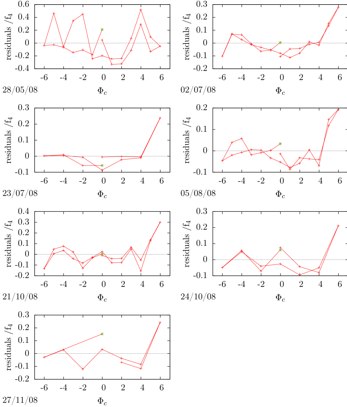
Figure 3.13: Residuals of the F_0 fit for the asymmetric calibrations. These residuals are calculated as (\arcsin \frac{F_{A,j}^+ - F_0}{K} - \arcsin \frac{F_{A,j}^- - F_0}{K} - \bar{\Psi}) \times K as described in (see (2.57) and (2.58)) on page 81. The asymmetry \Phi_c = \arcsin \frac{F_{A,j}^+}{K} - \arcsin \frac{F_{A,j}^-}{K} is illustrative; it does not enter the calculation. The lines mark the order of acquisition, the first point is marked differently.
