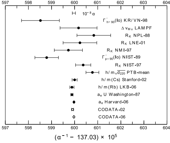
Figure 1.1: Values of the fine-structure constant \alpha with u_r < 10^{-7} , in order of decreasing uncertainty from top to bottom, and the 2002 and 2006 CODATA recommended values of \alpha . Data and Graph from [CoData06].
