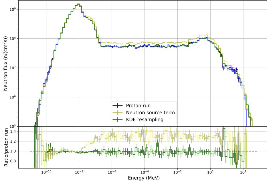
Figure 22: Neutron fluxes obtained from runs employing a proton source, the neutron source term and KDE resampling. The fluxes are measured at the exit of the monolith guide, 5.5 m from the moderator.
