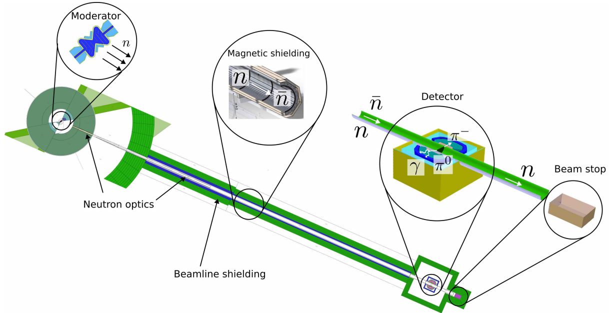
Figure 1: Conceptual overview of one of the proposed experiments to be performed at the HIBEAM beamline, namely neutron-antineutron oscillation searches. Neutrons emanating from the moderator may, in a magnetically shielded beamline, oscillate into antineutrons. Upon annihilation in a carbon foil, a final state of charged pions and photons may be observed in the surrounding detector system. A beam stop absorbs the remaining neutron beam. The figure features the PHITS beamline model and Geant4 detector model, both of which were constructed as a part of this thesis.
