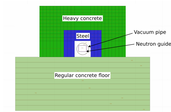
Figure 14: Cross-sectional view of the beamline just outside the bunker, showing the usage of steel and heavy concrete around the vacuum pipe.
