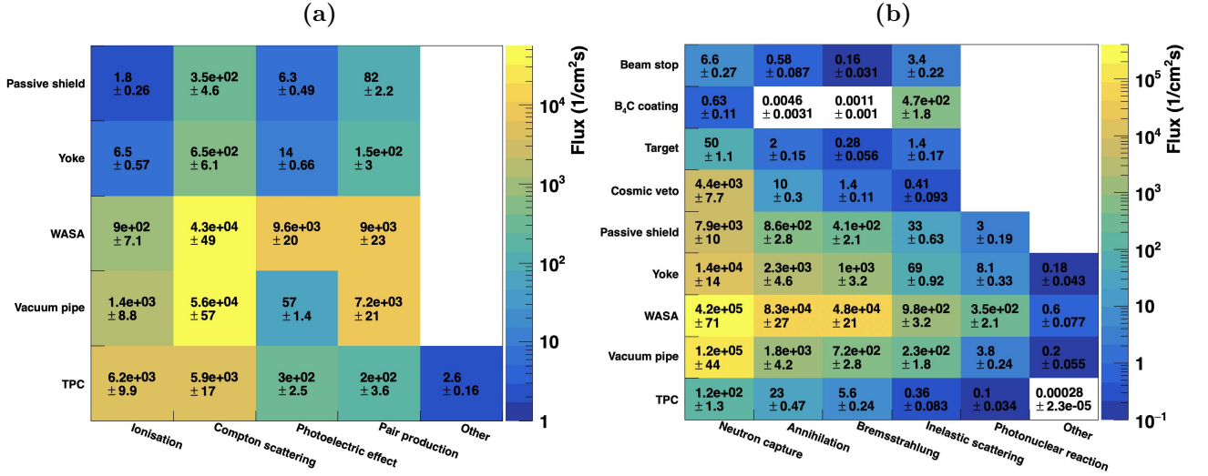
Figure 37: The particle flux in particles/(cm 2 ·s), subdivided into originating volume on the vertical axis and originating physics process on the horizontal axis. The results are obtained from Geant4 simulation. The shown uncertainties are statistical. Panel (a): For electrons in the TPC. Panel (b): For photons in the WASA calorimeter.
