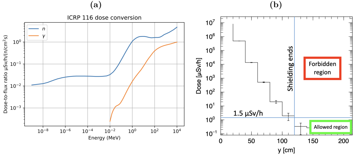
Figure 17: Panel (a): Worst-case flux-to-dose conversion coefficients of ICRP 116 for neutrons and photons. Panel (b): A dose map projection at x = 50 m from the moderator. The relevant dose rate limit is indicated by the horizontal blue line.
