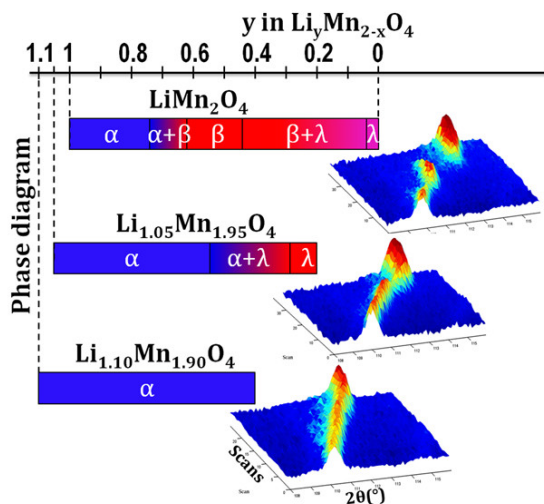
Figure 4: Phase transitions in spinel electrode materials subject to an electrical charge-and-discharge cycle. Reprinted with permission from [38]. © 2014, American Chemical Society.
